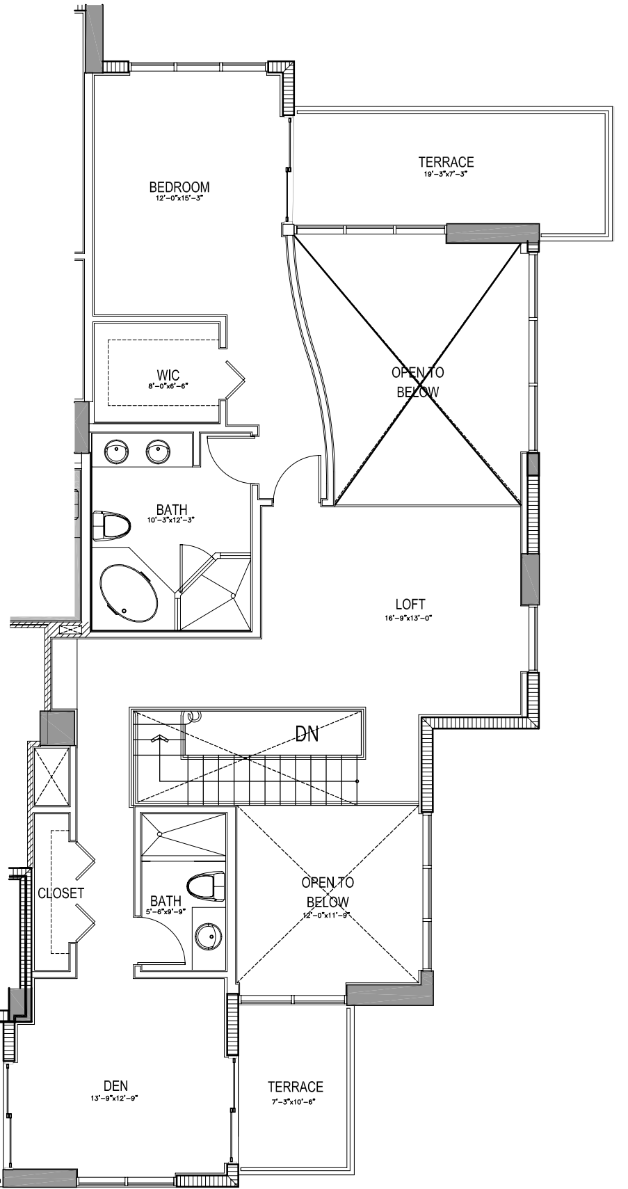
UPPER LEVEL
